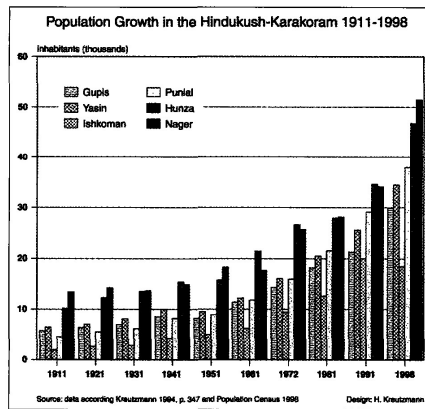
Fig. 42. Population growth in northern Pakistan.
